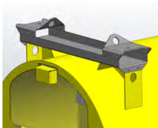
DE-MOUNT TOP BRACKETS AND FORKLIFT POCKETS
